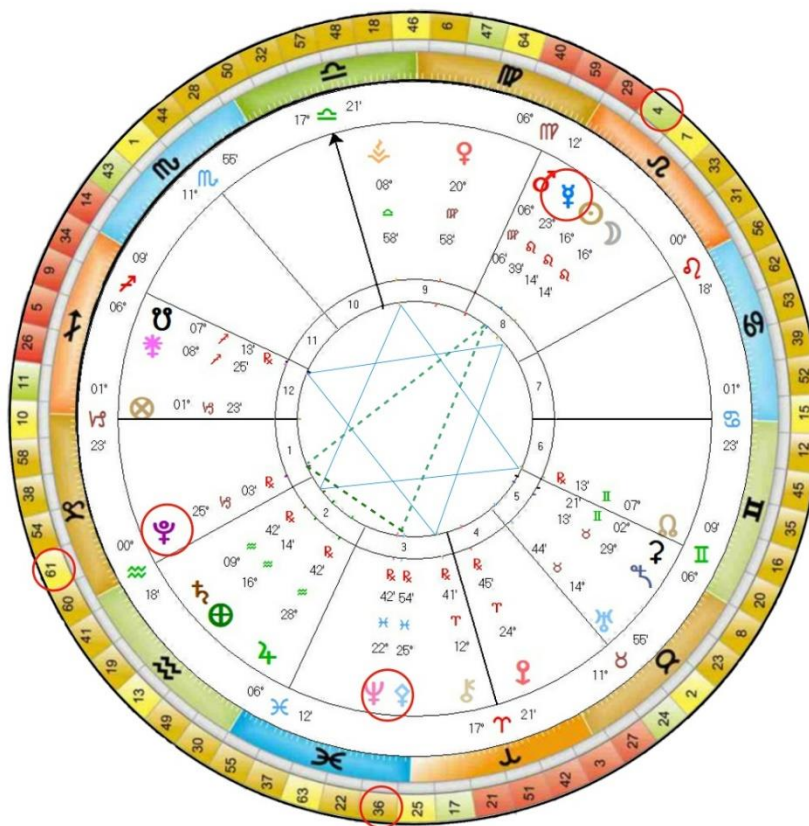
Chart for the Leo New Moon on 8.8.2021 at 15:55 EET Giza Egypt https://www.timeanddate.com/moon/phases
