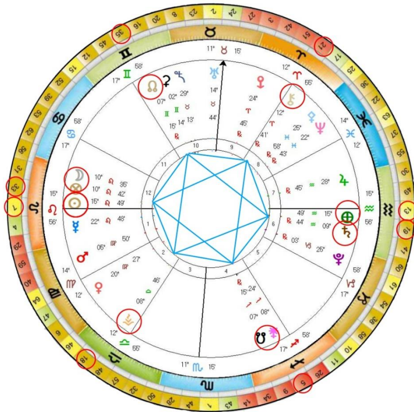
Chart for Sun Rising at the same time as Sirius 'The Lion's Gate' on 8.8.2021 at 05:23 EET Giza
